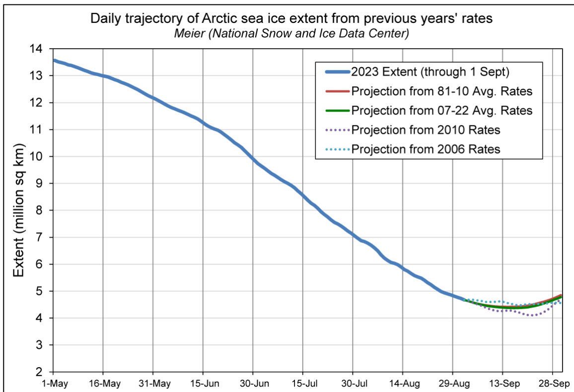
Figure 1. Predicted Arctic trajectories from the 1 September observed extent. The official estimate is based on the projection used the average of the last 16 years (2007-2022, green solid line) and for the 1981-2010 average (solid red line). The rates for 2006 and 2010 (dotted lines) yield the highest and lowest predicted extents respectively.
