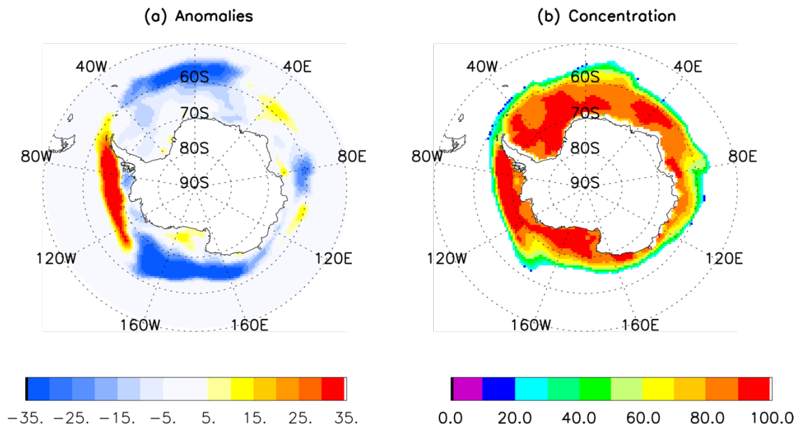
Figure 3 One-month lead prediction of September 2023 Antarctic sea ice concentration anomaly (a) and concentration (b) by a linear Markov model initialized with observed August SIC, SAT, GH300 and vector winds at 300mb.
