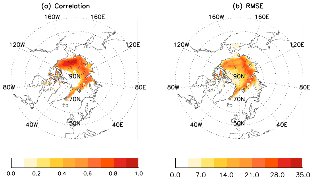
Figure 4. Cross-validated model skill measured by correlations between model predictions and observations of Arctic sea ice concentration anomalies (a) and model RMSE (b) for one-month lead prediction of September sea ice concentration. Only the correlations that pass the 95% confidence level are shown in (a). The units in (b) are in percentages. The low correlations and low RMSE near the North Pole Hole (the satellite blind spot) are due to low ice variability (Yuan et al. 2016).
