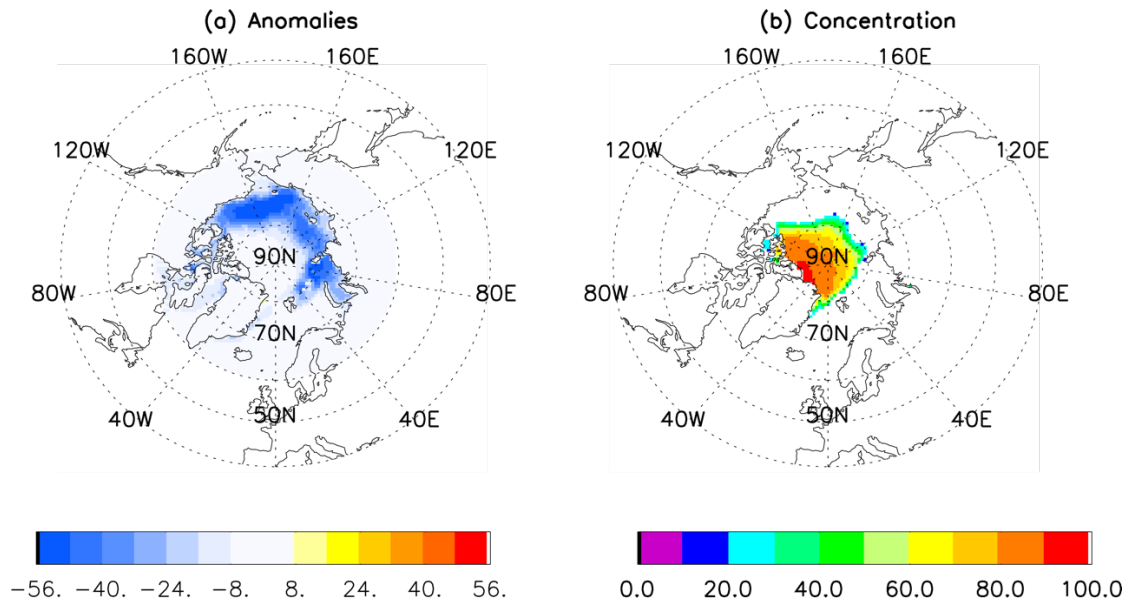
Figure 1 One-month lead prediction of 2023 September Arctic sea ice concentration anomaly (a) and concentration (b) by the linear Markov model initialized with observed August SIC, SST, SAT, GH300 and vector winds at 300mb.
