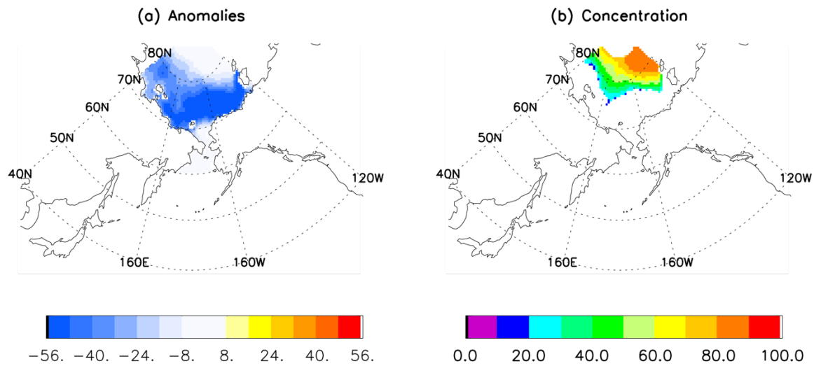
Figure 2 One-month lead prediction of September 2023 sea ice concentration anomaly (a) and concentration (b) in the Alaskan region by a regional linear Markov model initialized with observed August SIC, SST, SAT, GPH and winds at 500mb and 200mb.
