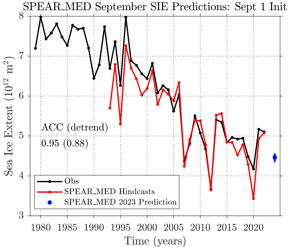
Figure 1: September pan-Arctic sea ice extent predictions from the GFDL-SPEAR_MED model initialized on September 1 (red dots) compared to NSIDC observations (black dots). The blue circles show the September 2023 predictions from the 30 ensemble members. The model predictions have been bias corrected via a linear-regression adjustment.
