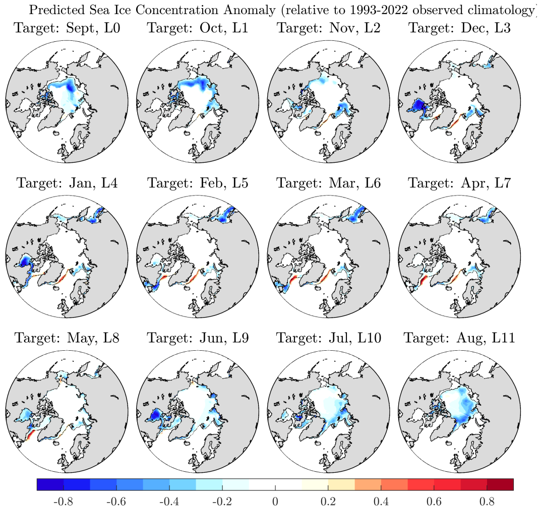
Figure 4: Monthly sea ice concentration anomaly predictions from the GFDL-SPEAR_MED model initialized on September 1. The anomalies are computed relative to the observed NSIDC NASA Team climatology over 1993–2022. The observed climatological sea ice edge position is shown in black. No bias correction has been applied.
