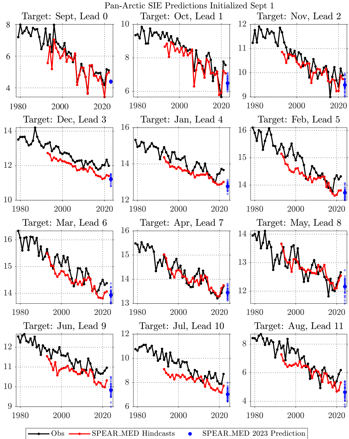
Figure 3: Monthly pan-Arctic sea ice extent predictions from the GFDL-SPEAR_MED model initialized on September 1 (red dots) compared to NSIDC observations (black dots). The blue circles show predictions from the 30 ensemble members. The model predictions have not been bias corrected.
