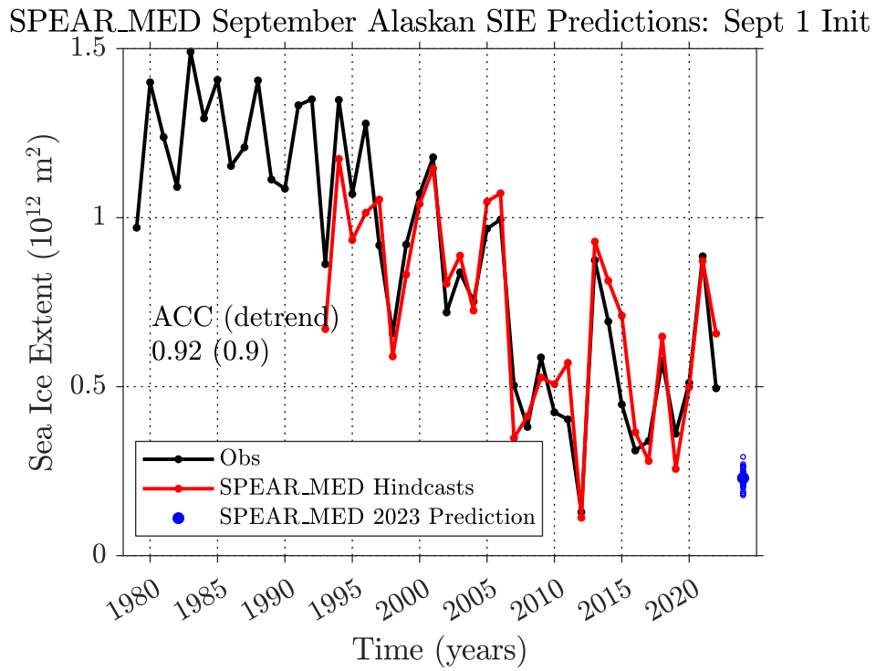
Figure 6: September Alaskan sea ice extent predictions from the GFDL-SPEAR_MED model initialized on September 1 (red dots) compared to NSIDC observations (black dots). The blue circles show the September 2023 predictions from the 30 ensemble members. The model predictions have been bias corrected via a linear-regression adjustment.
