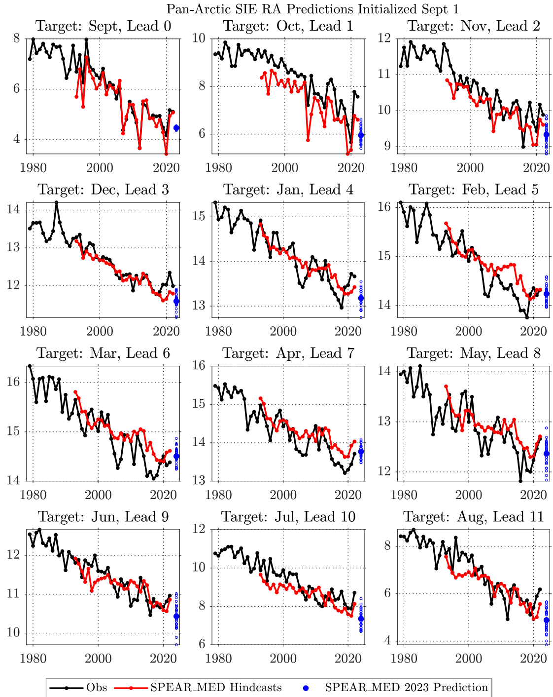
Figure 2: Monthly pan-Arctic sea ice extent predictions from the GFDL-SPEAR_MED model initialized on September 1 (red dots) compared to NSIDC observations (black dots). The blue circles show predictions from the 30 ensemble members. The model predictions have been bias corrected via a linear-regression adjustment.
