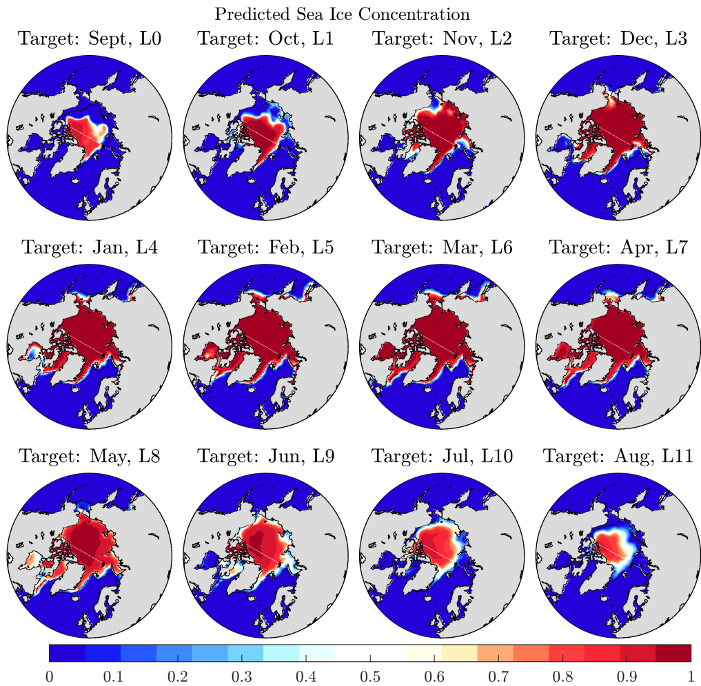
Figure 5: Monthly sea ice concentration predictions from the GFDL-SPEAR_MED model initialized on September 1. The observed climatological sea ice edge position is shown in black. No bias correction has been applied.
