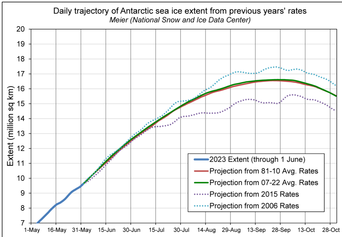
Figure 2. Predicted Antarctic trajectories from the 1 June observed extent. The official estimate is based on the projection used the average of the last 16 years (2007-2022, green solid line) and for the 1981-2010 average (solid red line). The rates for 2006 and 2015 (dotted lines) yield the highest and lowest predicted extents respectively.
