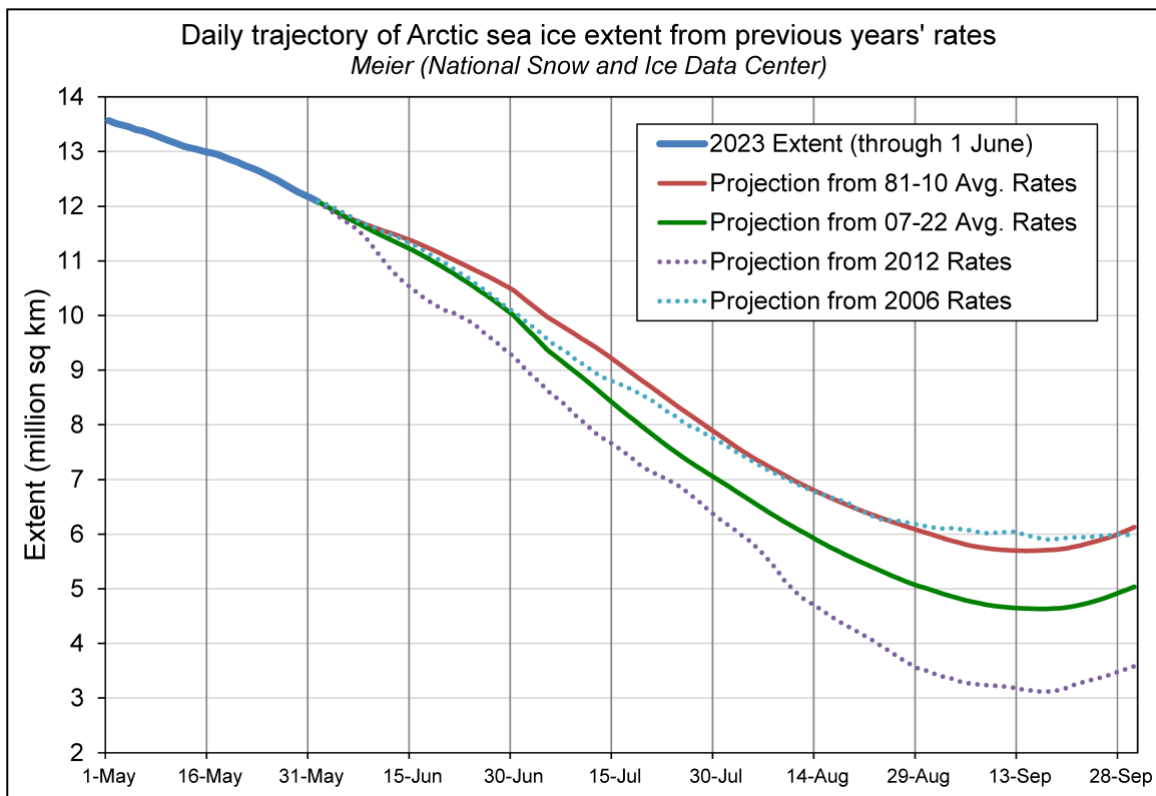
Figure 1. Predicted Arctic trajectories from the 1 June observed extent. The official estimate is based on the projection used the average of the last 16 years (2007-2022, green solid line) and for the 1981-2010 average (solid red line). The rates for 2006 and 2012 (dotted lines) yield the highest and lowest predicted extents respectively.
