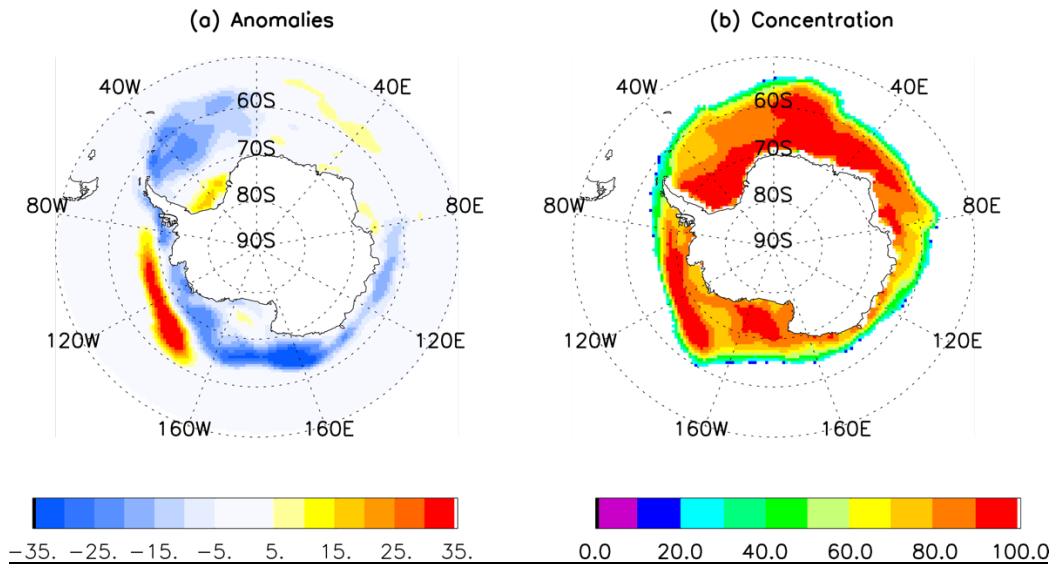
Figure 3 Two-month lead prediction of September 2023 Antarctic sea ice concentration anomaly (a) and concentration (b) by a linear Markov model initialized with observed July SIC, SAT, GH300 and vector winds at 300mb.
