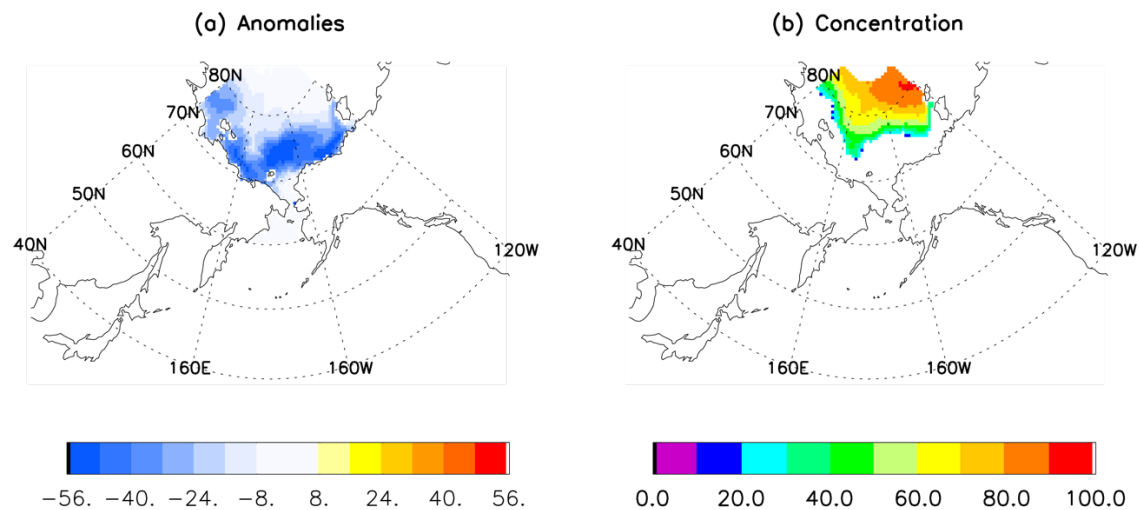
Figure 2 Two-month lead prediction of September 2023 sea ice concentration anomaly (a) and concentration (b) in the Alaskan region by a regional linear Markov model initialized with observed July SIC, SST, and SAT.
