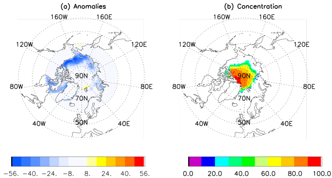
Figure 1 Two-month lead prediction of 2023 September Arctic sea ice concentration anomaly (a) and concentration (b) by the linear Markov model initialized with observed July SIC, SST, SAT, GH300 and vector winds at 300mb.
