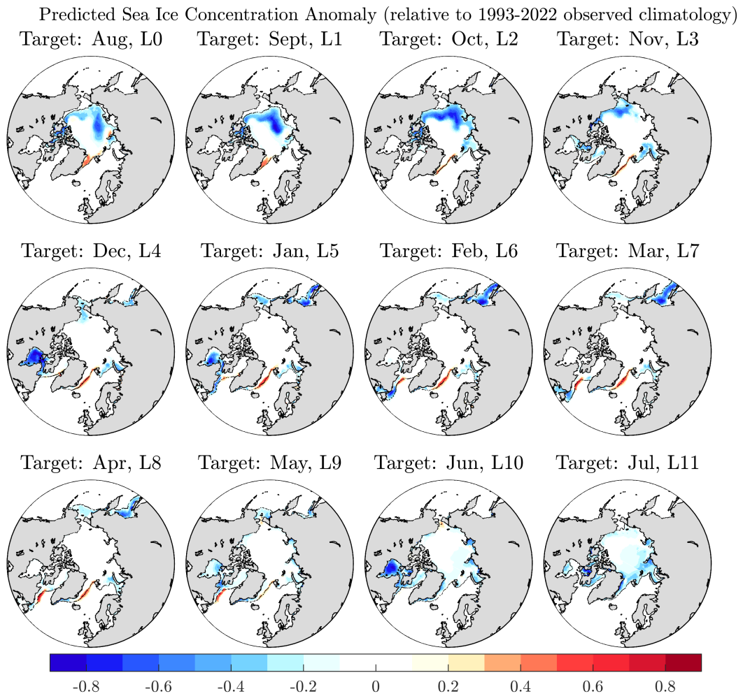
Figure 4: Monthly sea ice concentration anomaly predictions from the GFDL-SPEAR_MED model initialized on August 1. The anomalies are computed relative to the observed NSIDC NASA Team climatology over 1993–2022. The observed climatological sea ice edge position is shown in black. No bias correction has been applied.
