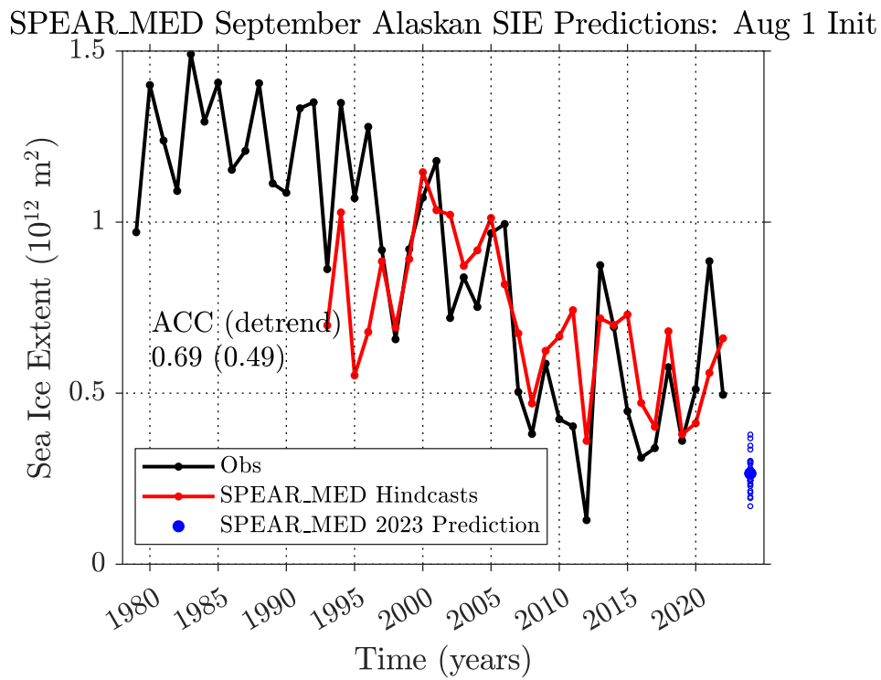
Figure 6: September Alaskan sea ice extent predictions from the GFDL-SPEAR_MED model initialized on August 1 (red dots) compared to NSIDC observations (black dots). The blue circles show the September 2023 predictions from the 30 ensemble members. The model predictions have been bias corrected via a linear-regression adjustment.
