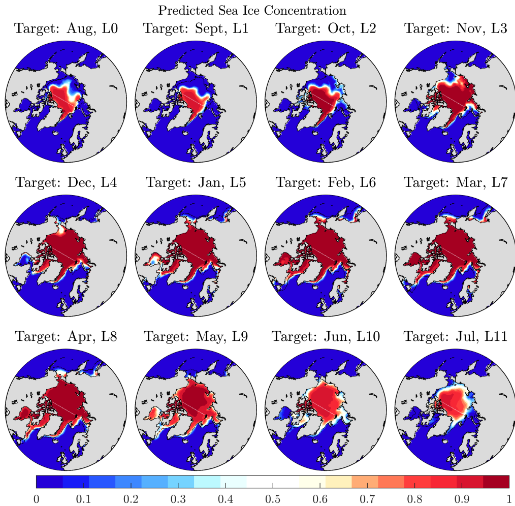
Figure 5: Monthly sea ice concentration predictions from the GFDL-SPEAR_MED model initialized on August 1. The observed climatological sea ice edge position is shown in black. No bias correction has been applied.
