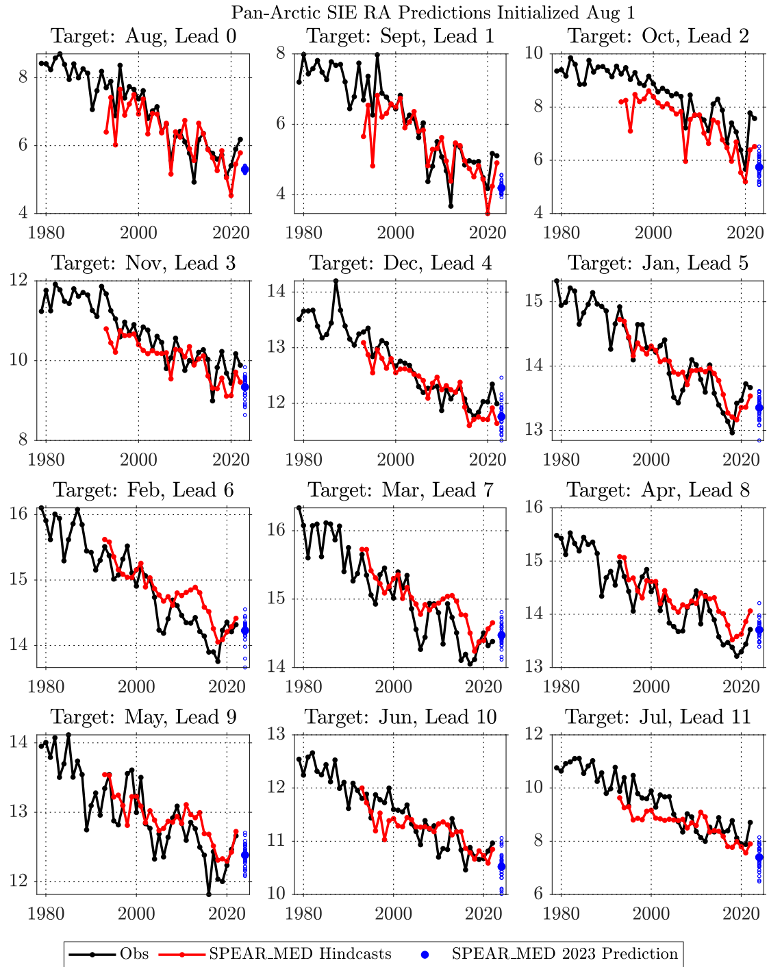
Figure 2: Monthly pan-Arctic sea ice extent predictions from the GFDL-SPEAR_MED model initialized on August 1 (red dots) compared to NSIDC observations (black dots). The blue circles show predictions from the 30 ensemble members. The model predictions have been bias corrected via a linear-regression adjustment.
