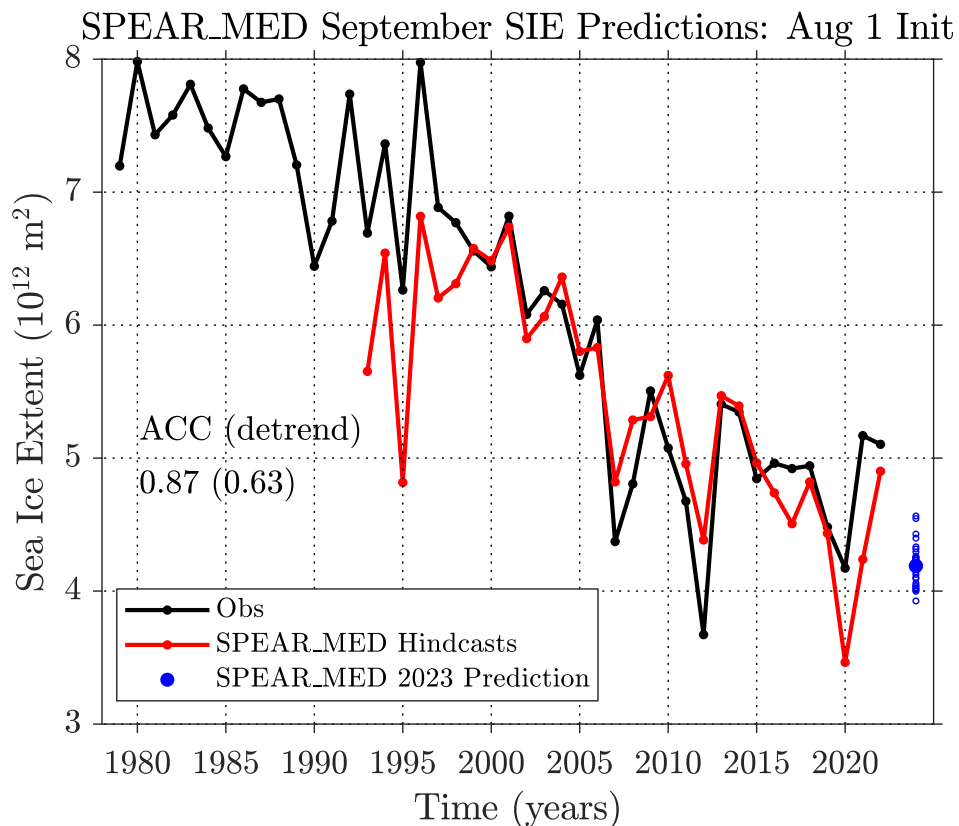
Figure 1: September pan-Arctic sea ice extent predictions from the GFDL-SPEAR_MED model initialized on August 1 (red dots) compared to NSIDC observations (black dots). The blue circles show the September 2023 predictions from the 30 ensemble members. The model predictions have been bias corrected via a linear-regression adjustment.
