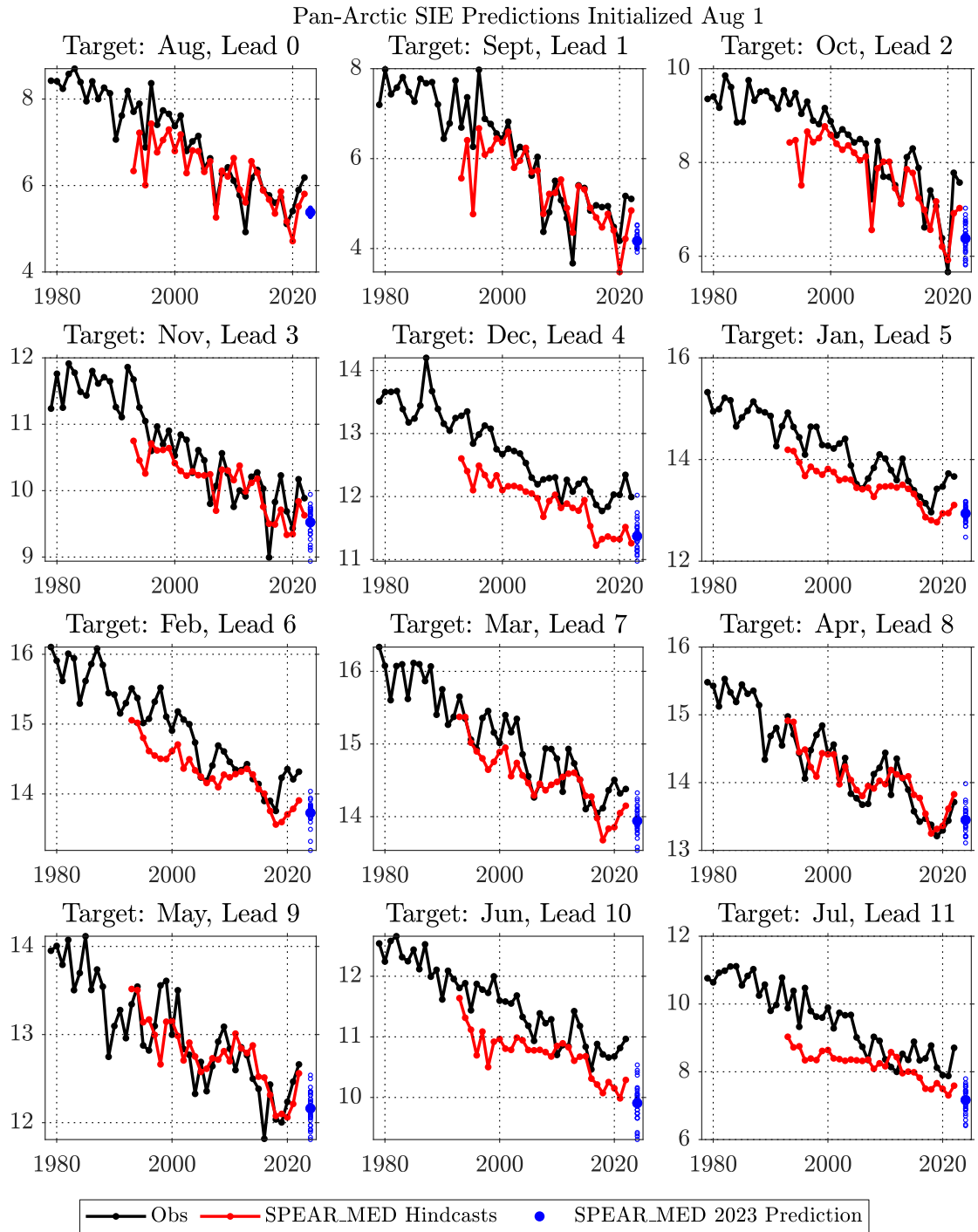
Figure 3: Monthly pan-Arctic sea ice extent predictions from the GFDL-SPEAR_MED model initialized on August 1 (red dots) compared to NSIDC observations (black dots). The blue circles show predictions from the 30 ensemble members. The model predictions have not been bias corrected.
