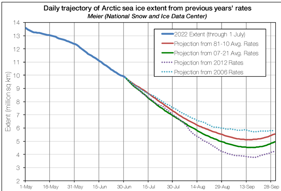
Figure 1. Predicted Arctic trajectories from the 1 July observed extent. The official estimate is based on the projection used the average of the last 15 years (2007-2021, green solid line) and for the 1981-2010 average (solid red line). The rates for 2006 and 2012 (dotted lines) yield the highest and lowest predicted extents respectively.
