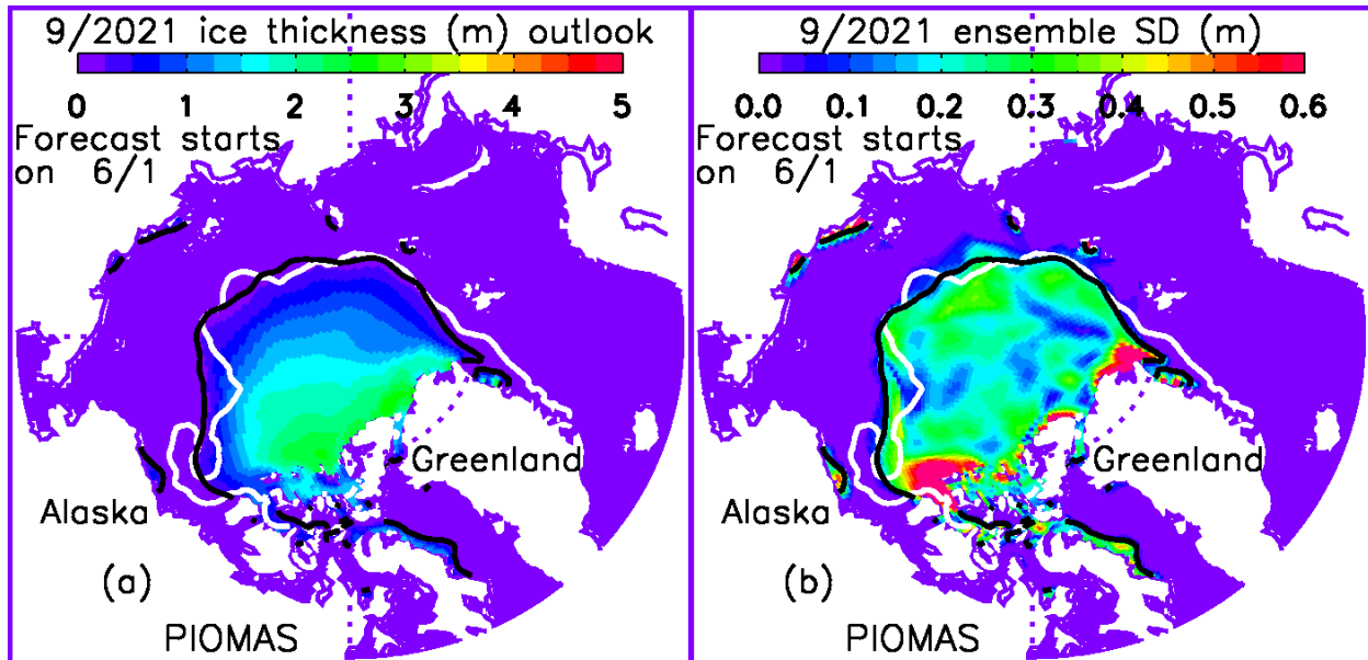
Figure 1. (a) Predicted Arctic September 2021 sea ice thickness and edge location (from ensemble mean), and (b) ensemble standard deviation (SD) of ice thickness which shows the uncertainty of the prediction. The white line represents the satellite-observed September 2020 ice edge defined as the line of 0.15 ice concentration, while the black line is the model predicted September 2021 ice edge.
