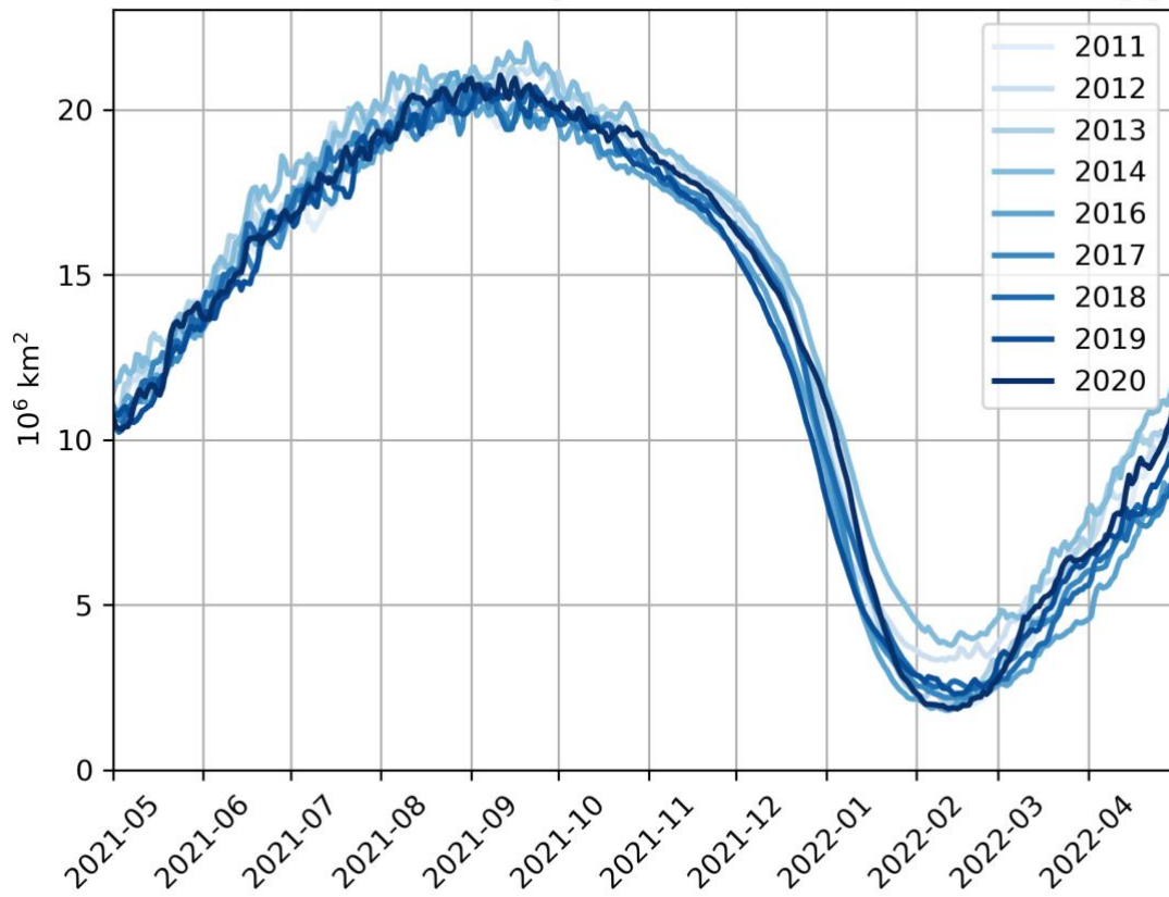
Predicted sea ice extent in region Antarctic with various forcing years
