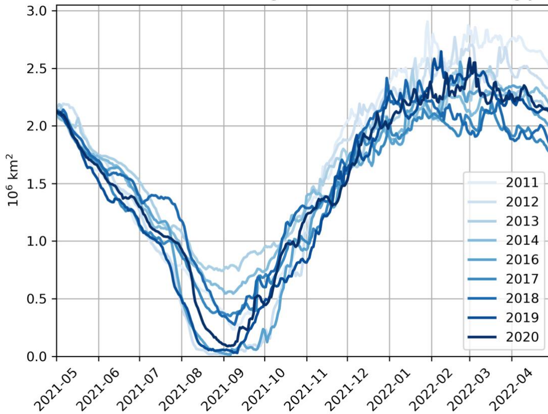
Predicted sea ice extent in region Alaska with various forcing years
