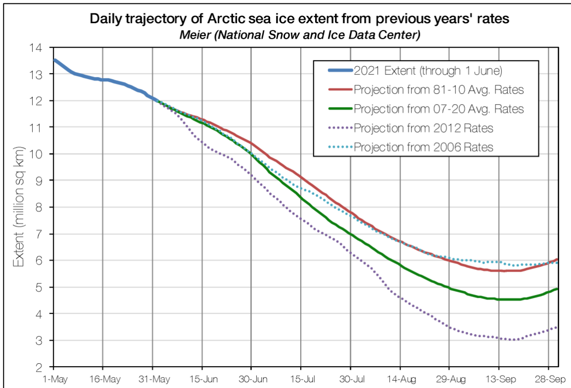
Figure 1. Predicted Arctic trajectories from the 1 June observed extent. The official estimate is based on the projection used the average of the last 16 years (2007-2020, green solid line) and for the 1981-2010 average (solid red line). The rates for 2006 and 2012 (dotted lines) yield the highest and lowest predicted extents respectively.
