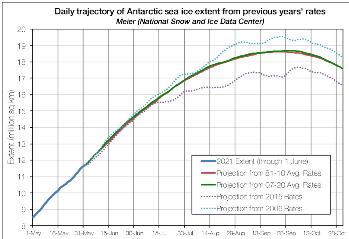
Figure 2. Predicted Antarctic trajectories from the 1 June observed extent. The official estimate is based on the projection used the average of the last 16 years (2007-2020, green solid line) and for the 1981-2010 average (solid red line). The rates for 2006 and 2015 (dotted lines) yield the highest and lowest predicted extents respectively.
