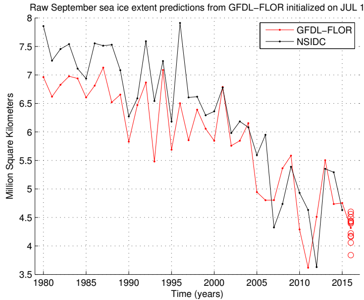
Figure 5: Same as Fig. 3, but without any bias correction applied to the model. The raw predictions have the same correlation with observations ( r=0.89 ), but a larger RMSE (0.63 million km 2 ) compared with the bias-corrected predictions (0.49 million km 2 ).
