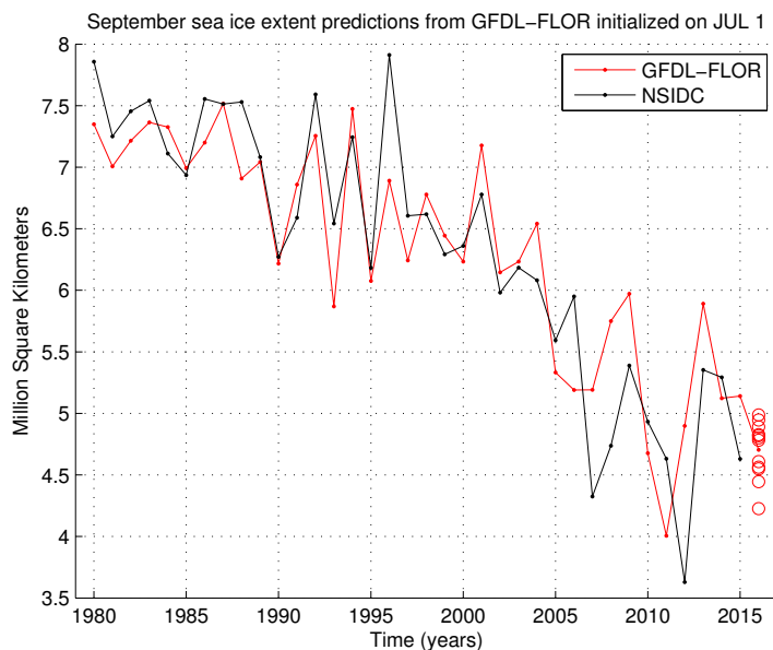
Figure 3: September pan-Arctic sea ice extent predictions from the GFDL-FLOR model initialized on July 1 (red dots) compared to NSIDC observations (black dots). The red circles show the September 2016 predictions from the 12 ensemble members. Note that the model predictions have been bias corrected.
