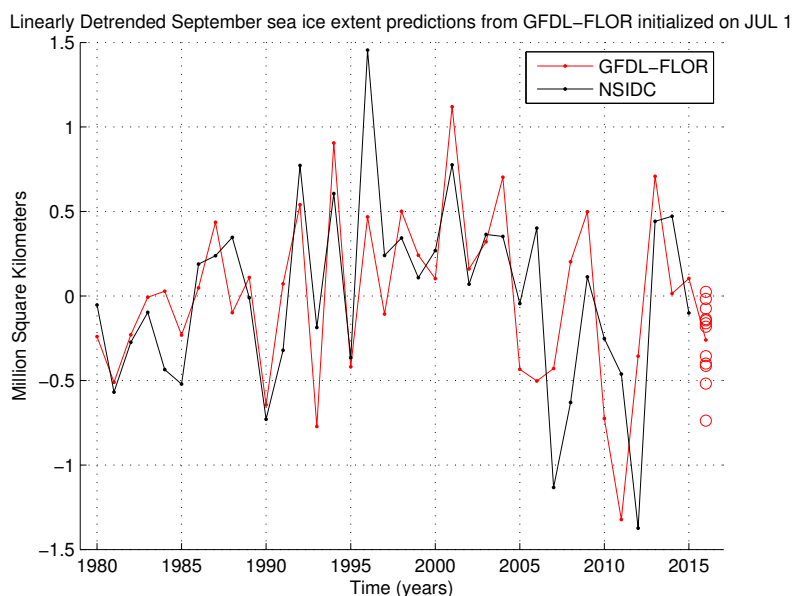
Figure 4: Linearly detrended September pan-Arctic sea ice extent predictions from the GFDL-FLOR model initialized on July 1 (red dots) compared to linearly detrended NSIDC observations (black dots). The red circles show the September 2016 predictions from the 12 ensemble members. The model has skill in predicting detrended extent ( r=0.63 ), in addition to the full extent field shown in Fig. 3 ( r=0.89 ).
