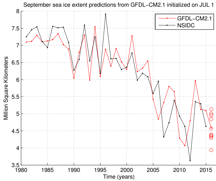
Figure 6: September pan-Arctic sea ice extent predictions from the GFDL-CM2.1 model initialized on July 1 (red dots) compared to NSIDC observations (black dots). The red circles show the September 2016 predictions from the 10 ensemble members. Note that the model predictions have been bias corrected.
