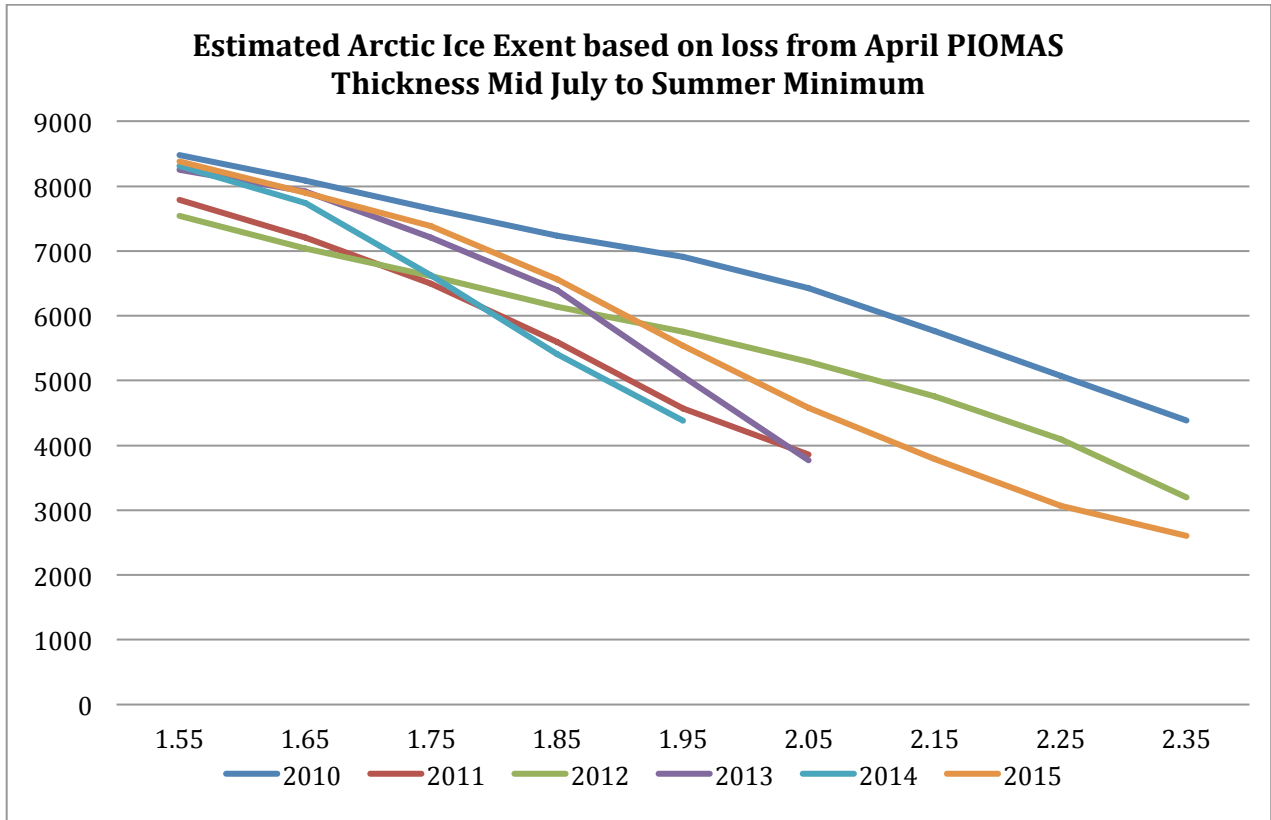
Graph 1: Predicted extent based on PIOMAS thickness loss July September
