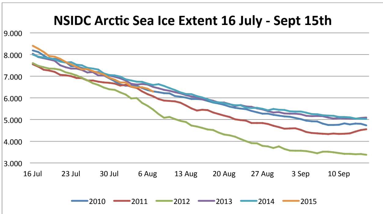
Graph 2: NSIDC extent July 16 th Sept 15th period
