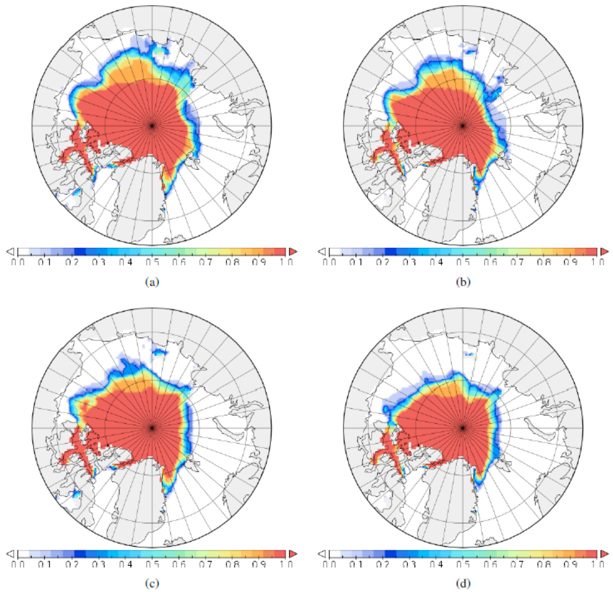
Figure 3: The probability in a grid cell to reach higher ice concentration than 15% (a) and c)) and the probability to reach higher ice thickness than 0.5m (b) and d)) for the ensemble run without initialization (a) and b)) and with initialization (c) and d)).
