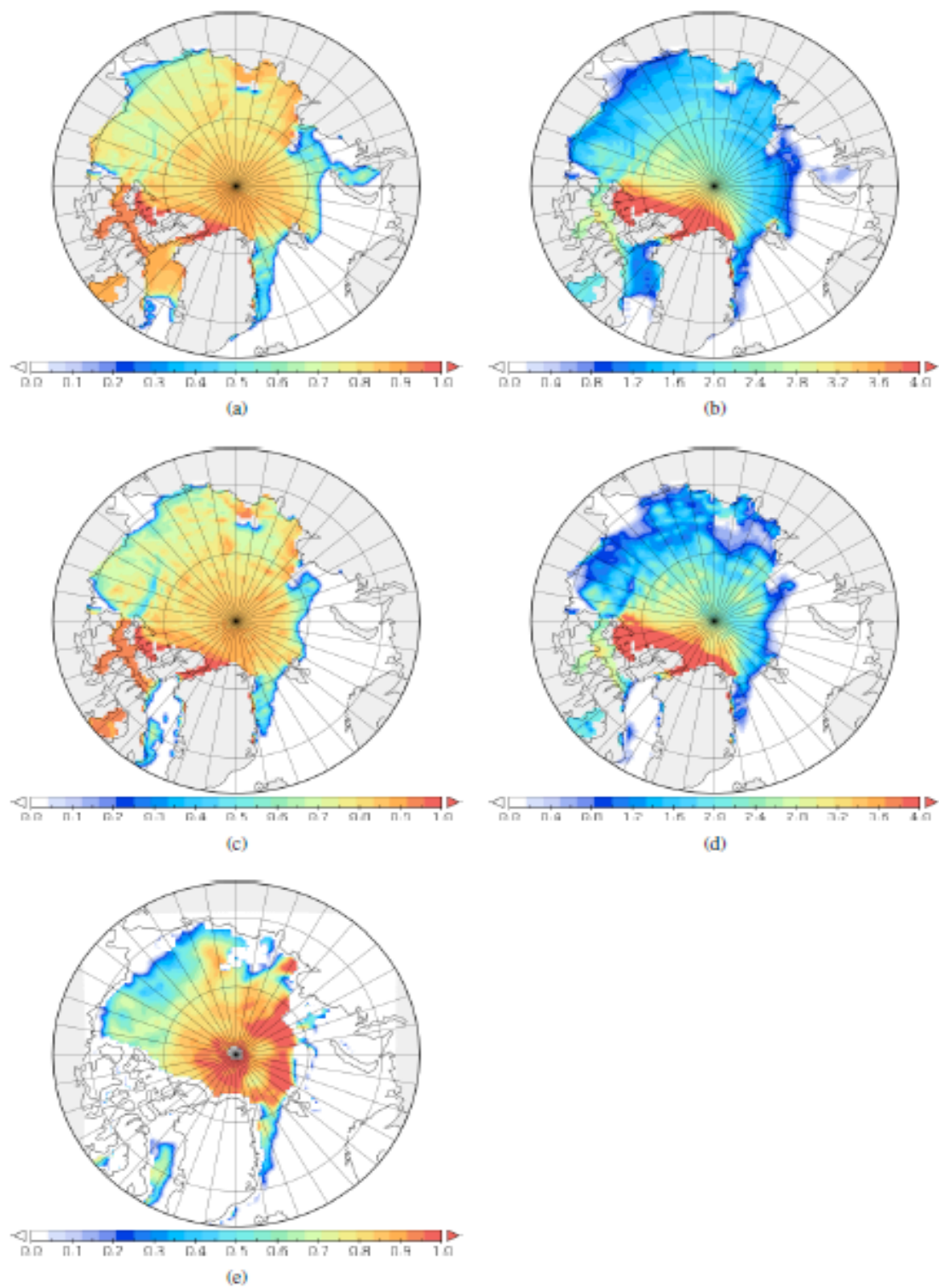
Figure 2: The modelled ice concentration [0-1] (a and c) and the ice thickness [m] (b and d) on July 7 2015 for the ensemble run without initialization (a and b) and with initialization (c and d). Additionally shown is the OSI SAF ice concentration on July 7 2015 (e).
