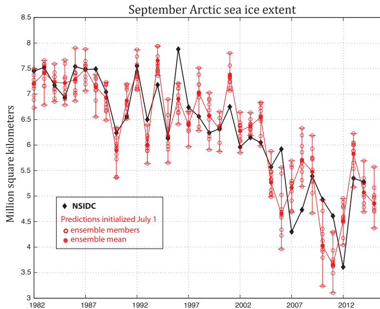
Figure 1: September Pan-Arctic sea ice extent in the GFDL CM2.1 predictions initialized July 1 (based on June data), compared to NSIDC observations. The ensemble means and the individual ensemble members are shown. The error bars indicate the lowest and highest extents in the 10-member ensemble. The model values have been bias-corrected.
