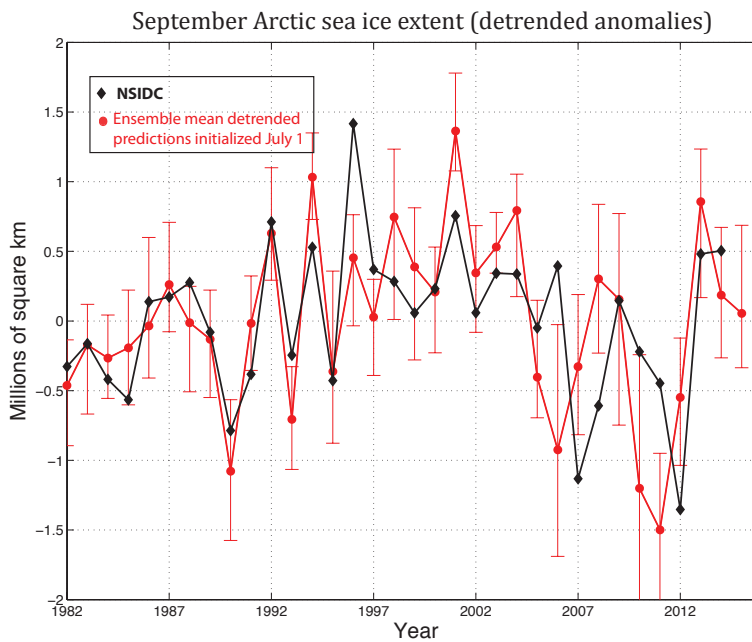
Figure 2: Comparison of detrended observations of September Arctic sea ice extent and detrended CM2.1 predictions initialized July 1. The error bars indicate the lowest and highest extents in the 10-member ensemble. The model values have been bias-corrected.
