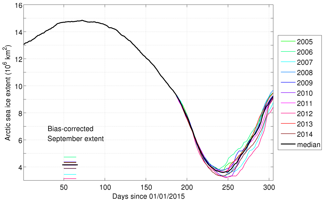
Figure 1: ensemble members and median 2015 daily Arctic sea ice extents. The bias-corrected September monthly mean extent for each member and their median (which is our final estimate) are also plotted as an inset.
