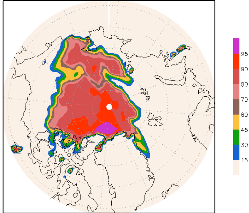
Ice Conc (%) Predicted for Sept 2015 w/ May IC
