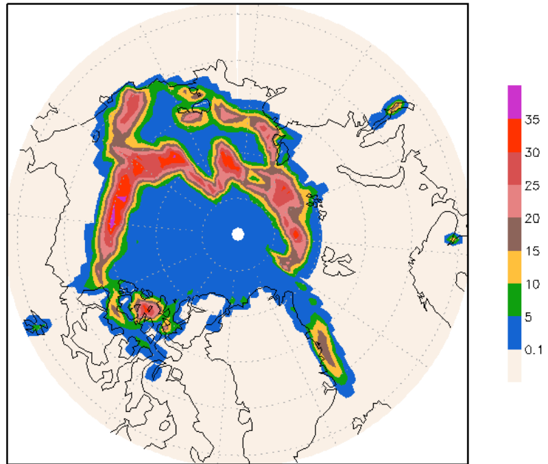
Ice Conc (%) S.D. for Sept 2015 w/ May IC
