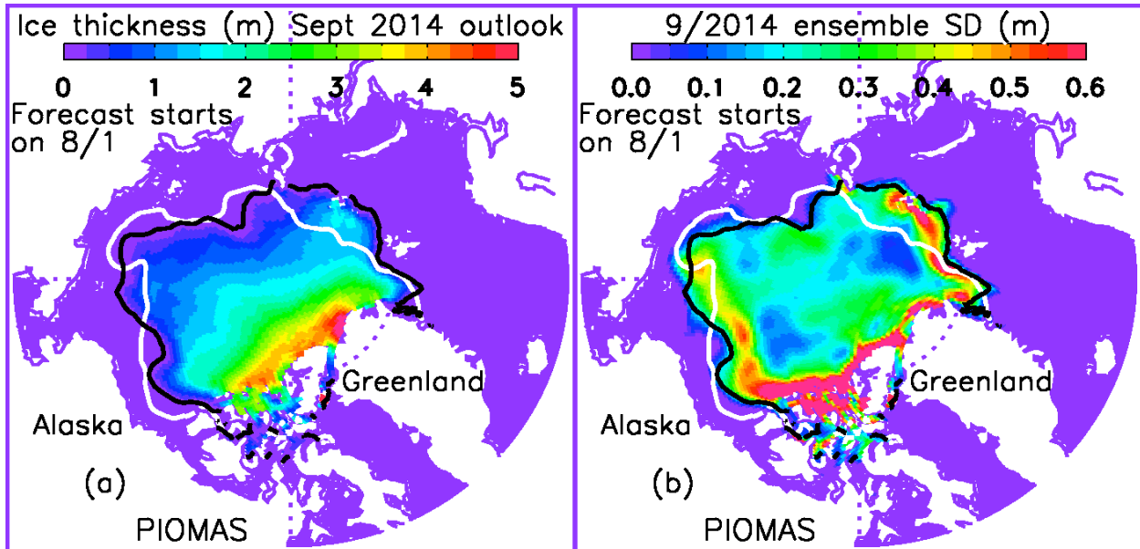
Figure 1. (a) Ensemble median prediction of September 2014 mean sea ice thickness and edge location, and (b) ensemble standard deviation (SD) of ice thickness which shows the uncertainty of the prediction. The white line represents the satellite-observed mean September 2013 ice edge defined as the line of 0.15 ice concentration, while the black line is the model predicted September 2014 ice edge.
