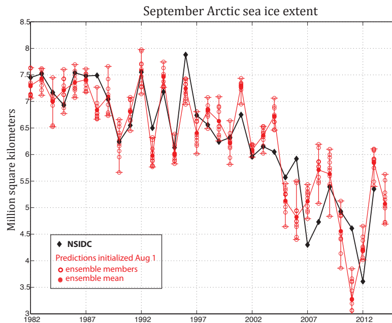
Figure 1: September Pan-Arctic sea ice extent in the GFDL CM2.1 predictions initialized August 1 (based on July data), compared to NSIDC observations. The ensemble means and the individual ensemble members are shown. The error bars indicate the lowest and highest extents in the 10-member ensemble. The model values have been bias-corrected.
