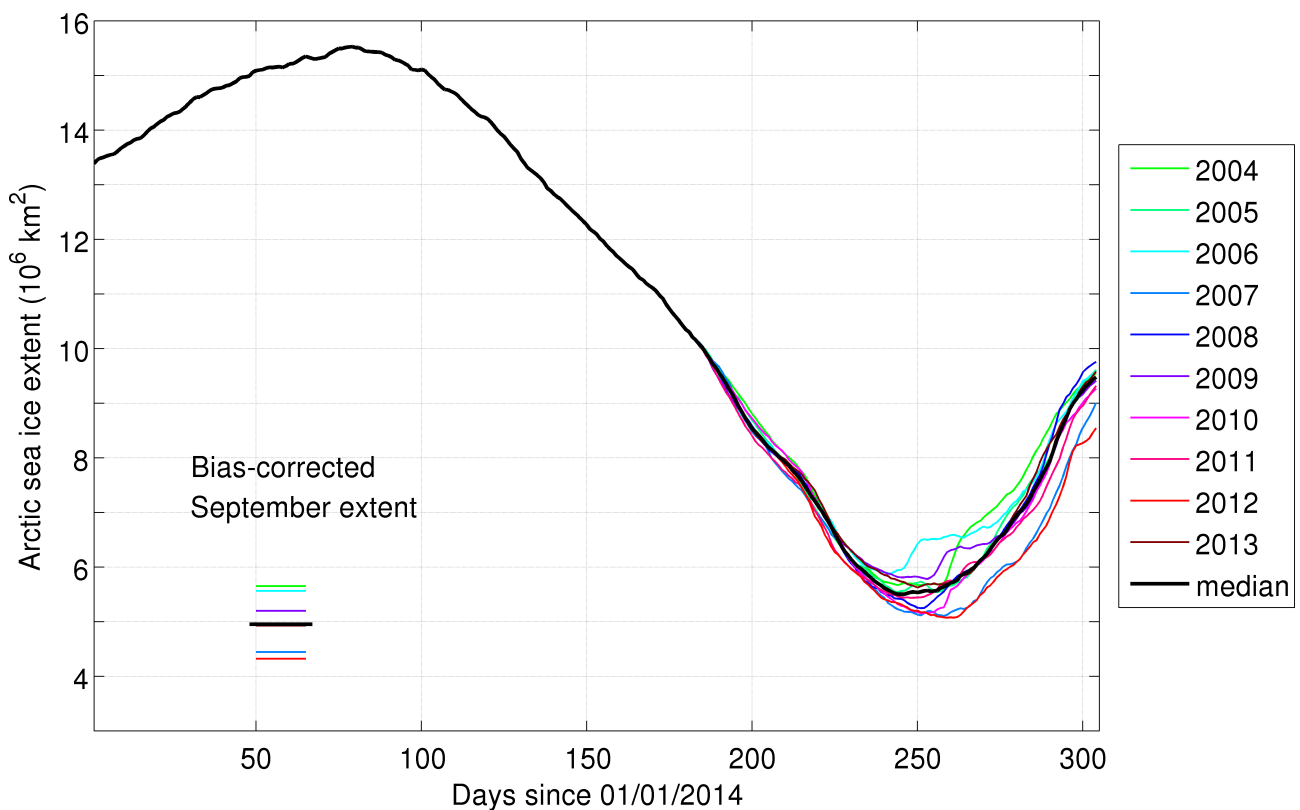
Figure: ensemble members and median 2014 daily Arctic sea ice extents. The bias-corrected September monthly mean extents for each members and their median (which is our final estimate) are also plotted as an inset.
