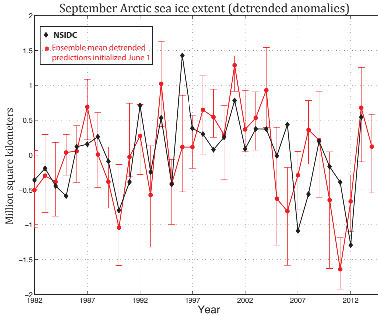
Figure 2: Comparison of detrended observations of September Arctic sea ice extent and detrended CM2.1 predictions initialized June 1. The error bars indicate the lowest and highest extents in the 10-member ensemble. The model values have been bias-corrected.
