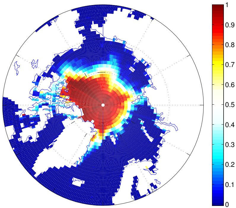
Figure 4: Sea ice concentration probability for September 2014
