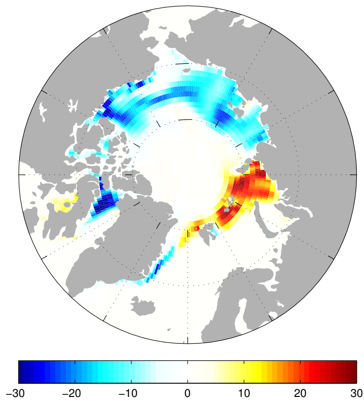
Figure 3: Difference in September sea ice concentration between the experiment and control ensembles in the GCM.
