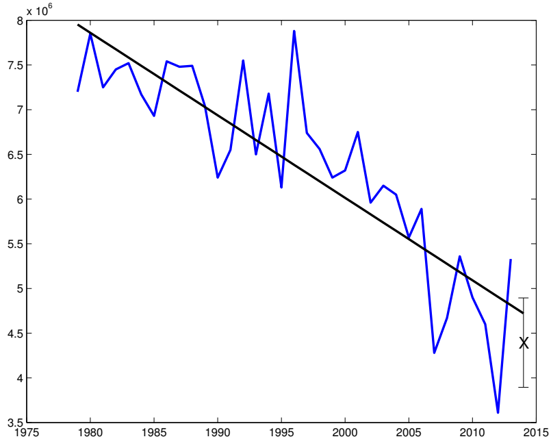
Figure 2: September sea ice extent in observations (1979-2013) together with a linear trend and 2014 forecast
