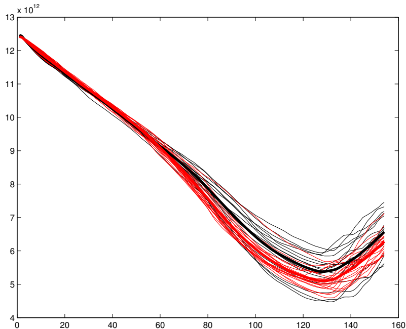
Figure 1: Daily sea ice area for the control (black) and experiment (red) ensembles. The mean for both ensembles is shown in bold.
